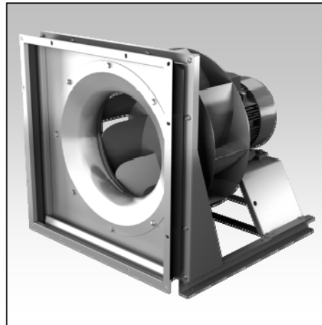
Free-running impellers as plug fan (IEC + EC)
