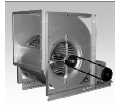
Single and Double inlet Belt driven fans (forward- and backward inclined)
